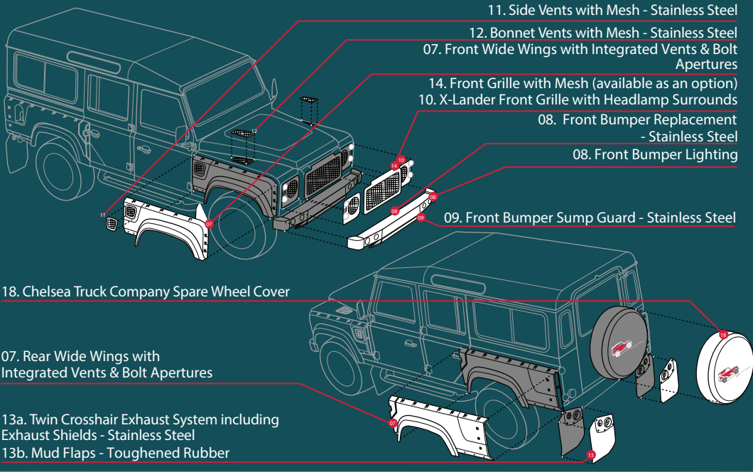
Defender 110 - Front & Rear Wider Wings with Integrated Vents & Bolt Apertures Carbon Composite 07 X - Lander Front Grille With Headlamp Surrounds 10
