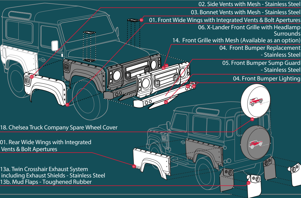
Front Bumper Replacement - Stainless Steel Includes Front Bumper Lighting Designed to Accommodate Original Bumper Mouldings.
